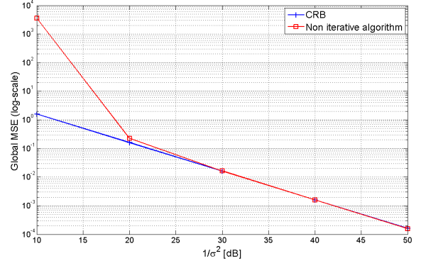
Fig. 2. Global MSE and \alpha\text{CRB} versus \frac{1}{\sigma^2} for one Hankel matrix and two unstructured matrices.
