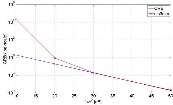
Fig. 1. Global MSE and \alpha\text{CRB} versus \frac{1}{\sigma^2} for three Toeplitz circulant matrices, I_1 = I_2 = I_3 = R = 5
