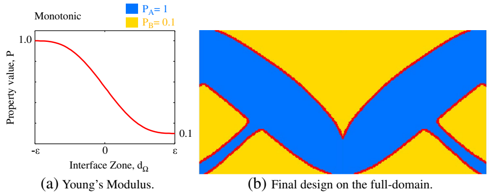
Fig. 6 Case for monotonic interface interpolation applied in the built-in-beam subjected to a point load (Fig. 5). Results shown on the half-domain unless otherwise noted. The design images show the distribution of materials A (blue) and B (yellow) in the domain, with the interface zone highlighted in red
