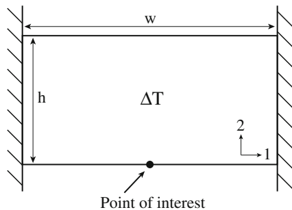
Fig. 14 The design problem for the built-in-beam with loading and boundary conditions. The analysis is thermoelastic with \Delta T=1
