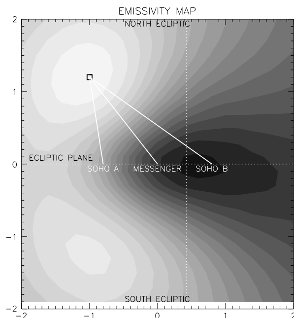
Figure 4. Explanation for the geometry of the observation in roll 37. The contour plot shows the volume emission rate derived from the model in the plane perpendicular to the ecliptic plane and containing the line passing through the positions of SOHO and MESSENGER. The axes are distances in AU. The X axis is this line passing by the positions of MESSENGER and SOHO. In this case, SOHO is behind MESSENGER (SOHO B). The corresponding position of SOHO ahead of MESSENGER (SOHO A) is shown too. The point at (0,0) is the point of the X axis closest to the Sun. The difference in intensities observed by SWAN and UVVS outside the ecliptic plane is caused by a parallax effect between MESSENGER and SOHO B. From this graph we see that SWAN measurements peak at lower latitude than UVVS measurements which is what is seen in the previous graph.
