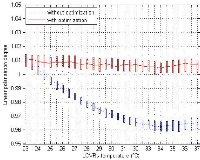
Fig. 5: Estimation of the polarization degree of a linearly polarized light wave as function of temperature
