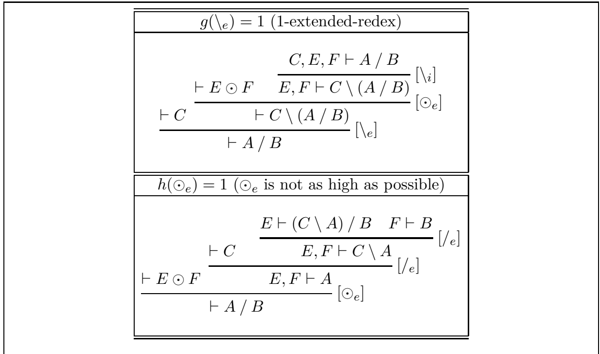
Figure 4: Examples of proof which are not in normal form
