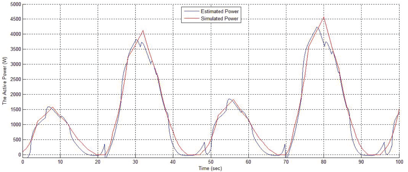
Fig. 12. The DF1G active power.
