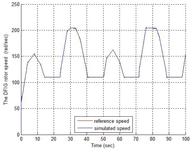
Fig. 11. The DF1G rotor speed and its reference.
