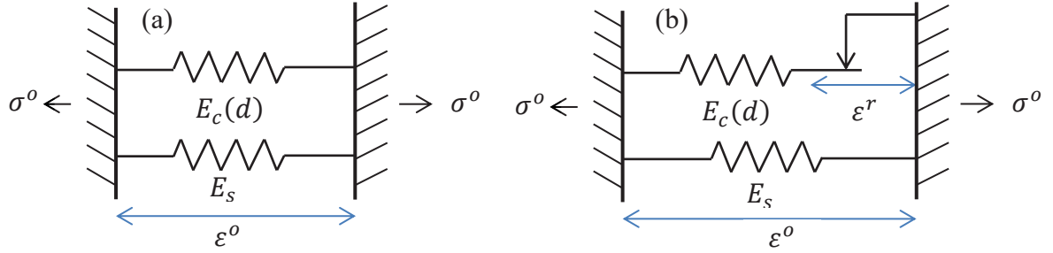
Figure 4: Associated rheological models for (a) the pure damage model and (b) the damage + crack opening model
