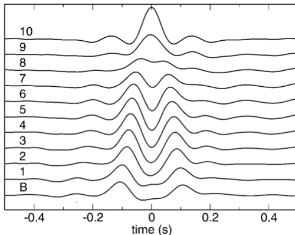
Figure 4: Seismic interferometry of the building computed at the Milikan Library by Snieder and Safak [SS06]
