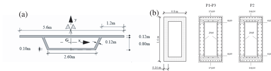
Figure 7: Viaduct: (a) deck, (b) piers (scale 1:2.5) [PVP+96].
