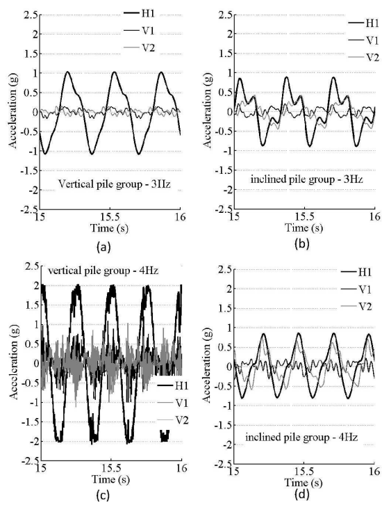
Figure 12: Kinematic reponse of the pile cap : effect of frequency input on the performances of inclined pile, [Esc12].
