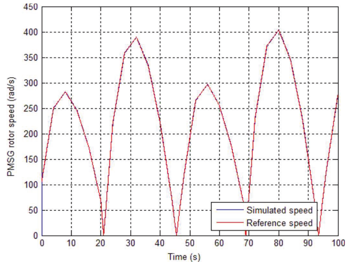
Fig. 10. PMSG rotor speed and its reference.
