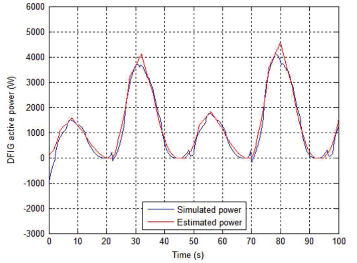
Fig. 9. DFIG active power.
