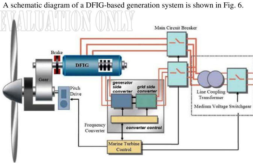
Fig. 6: Schematic diagram of a DFIG-based generation system
