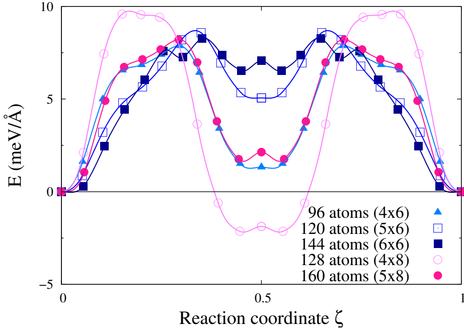
Figure 6: Energy barrier encountered by a screw dislocation dissociated in a prismatic plane when gliding in a pyramidal \pi_{1D} plane. Ab initio calculations are performed for different simulation cell sizes n \times m . (color online)
