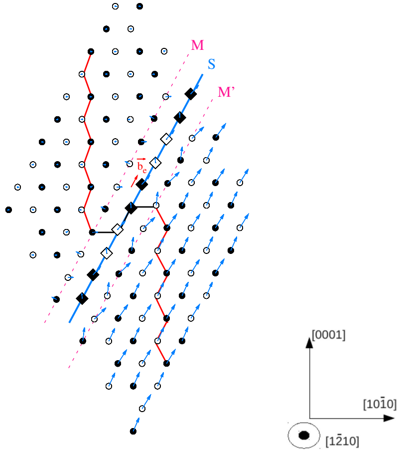
Figure 4: Atomic structure of the metastable pyramidal stacking fault: The displacement in the shearing \langle a \rangle = [1\bar{2}10] direction is shown by the projection of atoms in this direction, where atoms are sketched by black and white symbols depending on their position at half or full \langle a \rangle vector respectively. The blue arrows show atom displacements perpendicular to the shearing direction in the (1\bar{2}10) plane with a magnification factor of 3. The metastable fault corresponds to a pyramidal \{10\bar{1}1\} twin bordered by two mirror planes M and M' sketched by pink dashed lines. The blue line S corresponds to the shearing plane. The mirror planes symmetry is highlighted by a broken line corresponding to the corrugated prismatic plane, in red in the parent hcp crystal and in black in the twinned crystal. Atoms with a neighborhood corresponding to the twinned crystal are sketched by diamonds, while the circles corresponds to atoms in the parent crystal. (color online)
