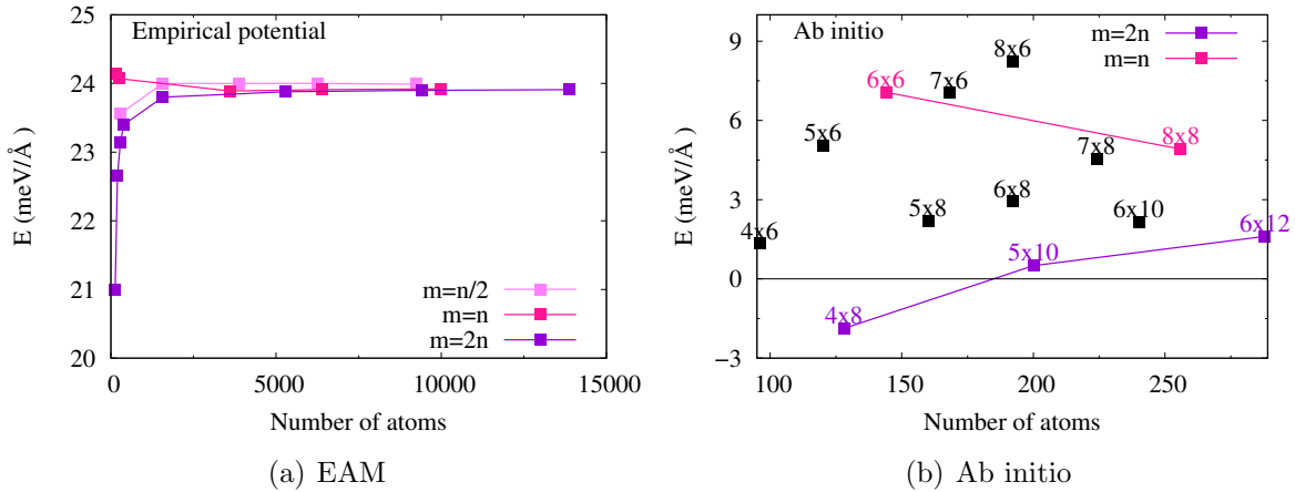
Figure 8: Difference between the energy of the metastable configuration and the equilibrium configuration of the screw dislocation for different simulation cell sizes n \times m obtained with the EAM potential on the left and with ab initio calculations on the right. (color online)
