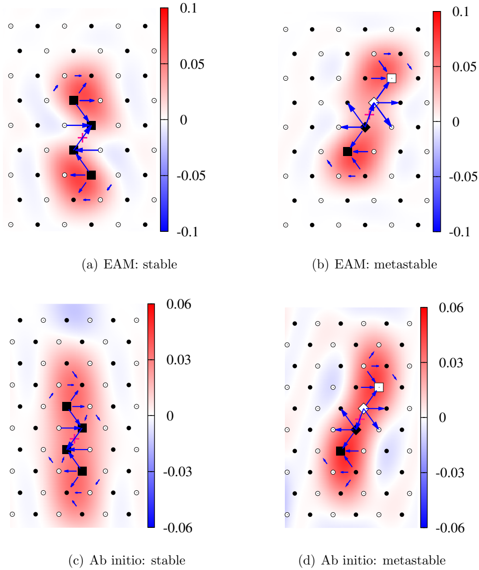
Figure 7: Differential displacement map of the screw dislocation in its equilibrium and metastable configuration deduced from ab initio calculations and EAM potential. The black and white symbols corresponds to atoms depending on their position along the \langle a \rangle = [1\bar{2}10] direction in the perfect crystal, while the blue arrows corresponds to the differential displacement between two columns of atoms in the \langle a \rangle direction after relaxation with dislocations. The pink cross indicates the dislocation center obtained by symmetry. The screw component of the Nye tensor distribution is superimposed. Squares correspond to atoms in a prismatic fault neighborhood while diamonds correspond to atoms in the pyramidal twin neighborhood. (color online)
