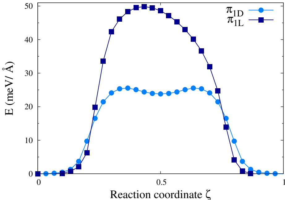
Figure 5: Energy barrier encountered by a screw dislocation dissociated in a prismatic plane and gliding in pyramidal \pi_{1L} and \pi_{1D} planes calculated with the EAM potential. (color online)
