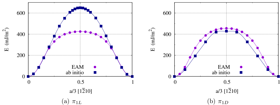
Figure 3: Generalized stacking fault energy in the first order pyramidal plane ( 10\bar{1}1 ) along the [\bar{1}2\bar{1}0] direction calculated with ab initio and with the EAM potential. The crystal is sheared either (a) in the loose plane \pi_{1L} , or (b) in the dense plane \pi_{1D} . (color online)
