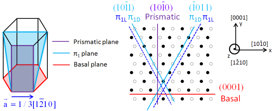
Figure 1: Hexagonal close-packed structure showing the different potential glide planes for a screw dislocation of Burgers vector \vec{a} = 1/3 [1\bar{2}10] . A projection perpendicular to \vec{a} is shown on the right, where atoms are sketched by circles with a color depending on their (1\bar{2}10) prismatic plane. (color online)
