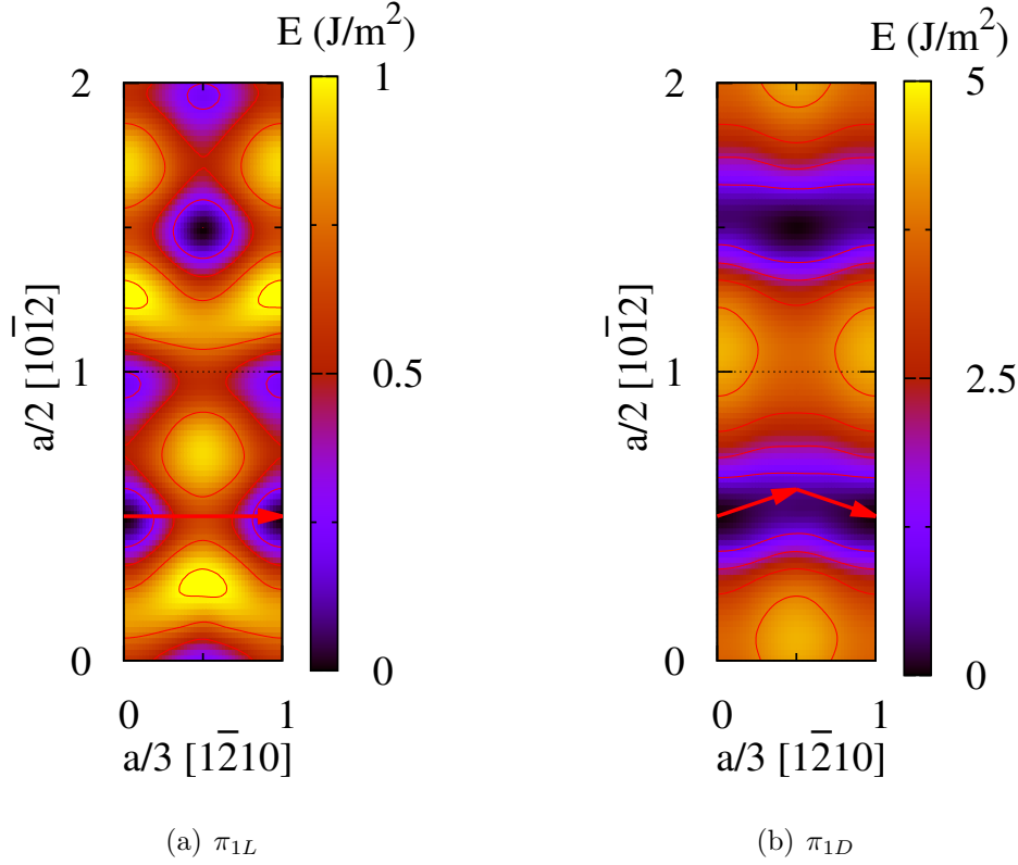
Figure 2: Generalized stacking fault energy in the first order pyramidal plane ( 10\bar{1}1 ) calculated with ab initio. The crystal is sheared either (a) in the loose plane \pi_{1L} , or (b) in the dense plane \pi_{1D} . The red arrows show the fault vector a/3 [1\bar{2}10] in (a) and its decomposition in (b) corresponding to the metastable stacking fault obtained after a full relaxation of atoms in the \pi_{1D} plane. (color online)
