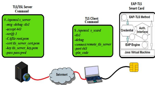
Fig. 3. The Platform design and experimental of “s_scared” command
