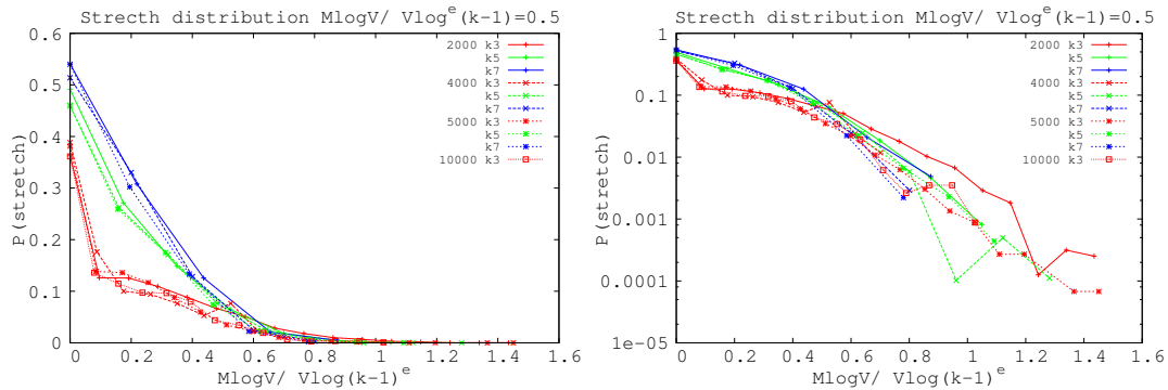
Figure 14: Stretch distribution. Left - The difference L^y - L_{shortest}^y is normalized and plotted for each communication in the dense regime for degrees k = 3, 5, 7 . For k = 3 we have 40% of communications correspond to the shortest paths while others take routes which are long compared to the average path length \log V / \log^\gamma(k-1) . In the case of higher connectivities k = 5, 7 there is a higher fraction of paths with the same length as the shortest path due to the routing flexibility offered. Right - The same data is plotted on a log scale to highlight the tails behavior.
