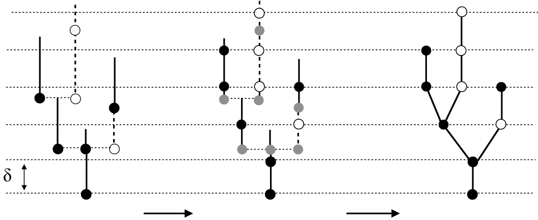
FIGURE 3. Discretisation of a two type tree with edge lengths.
