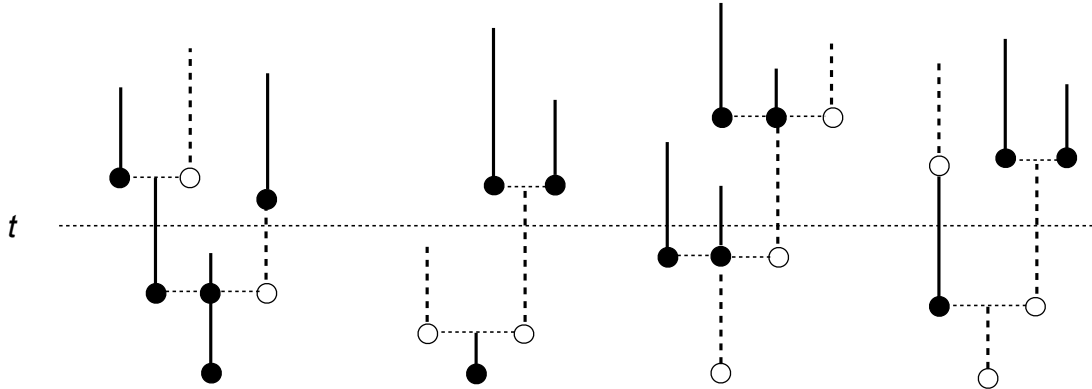
FIGURE 1. A two type forest with edge length issued from x = (2, 2) . Vertices of type 1 (resp. 2) are represented in black (resp. white). At time t , Z_t^{1,1} = 2 , Z_t^{1,2} = 2 , Z_t^{2,1} = 3 and Z_t^{2,2} = 4 .
