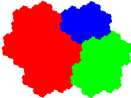
FIGURE 1. The classical Rauzy fractal.
