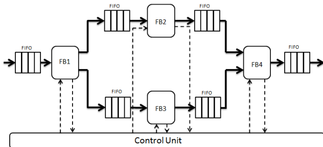
Fig. 2. Typical SDF dataflow RTL architecture.
