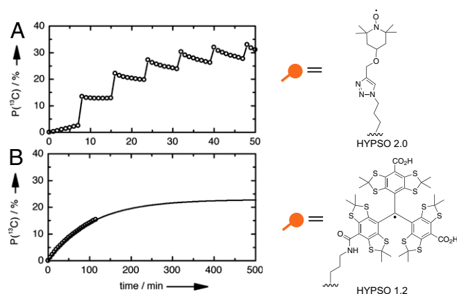
Fig. 3. (A) ^1\text{H} \rightarrow ^{13}\text{C} CP-DNP performed on 20 mg HYPISO 2.0 material (41 \mu\text{mol/g} ) impregnated with 36 \mu\text{L} 3 M solution of [ 1\text{-}^{13}\text{C} ]-pyruvate in \text{D}_2\text{O} . P(^{13}\text{C}) > 30\% is reached in 32.5 min with ^1\text{H} \rightarrow ^{13}\text{C} CP applied at 7.5-min intervals. (B) Direct ^{13}\text{C} DNP performed on 20 mg HYPISO 1.2 material (16 \mu\text{mol/g} ) impregnated with 36 \mu\text{L} 3 M solution of [ 1\text{-}^{13}\text{C} ]-pyruvate in \text{D}_2\text{O} . P(^{13}\text{C}) = 15\% is achieved after 2 h with a monoexponential buildup time \tau_{\text{DNP}}(^{13}\text{C}) = 104.6 \pm 2.4 min, potentially toward a maximum P(^{13}\text{C})^{\text{max}} = 22.9\% . Note that the horizontal scale has been extended by a factor of 10 for B with respect to A. Schematic representations of the radicals in the materials are given in A, Right and B, Right.
