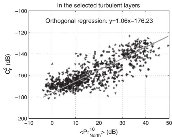
Figure 7. Pr_{\text{North}}^{10} versus moist C_n^2 (dB) (shown in Figure 6d). The solid gray line is the result of a linear fitting using an orthogonal regression.
