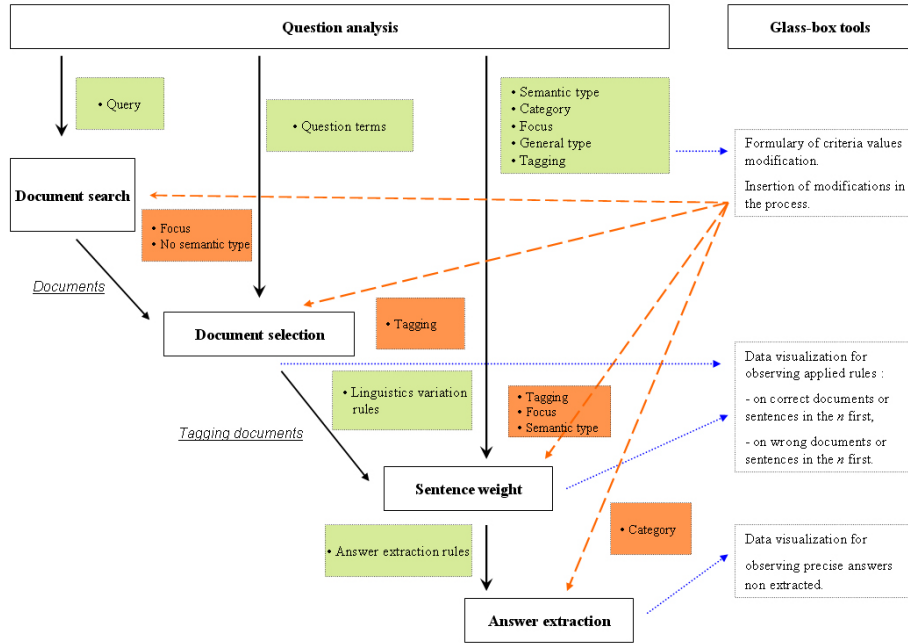
Fig. 1. Glass-box evaluation
