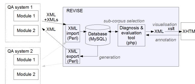
Figure 1: REVISE architecture
