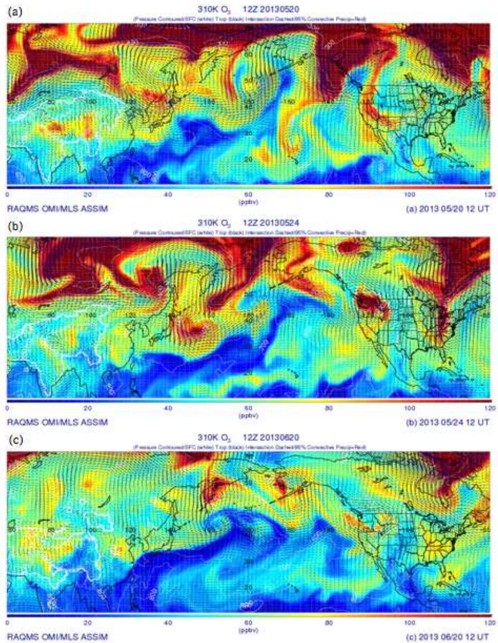
4 5 6 Figure 11. RAQMS O 3 analyses for the 310K isentropic surfaces at 1200 UT on: (a) May 7 20, (b) May 24, and (c) June 20, 2013 showing the midlatitude cyclones over the Pacific 8 Northwest responsible for the stratospheric intrusions detected above Angel Peak.
