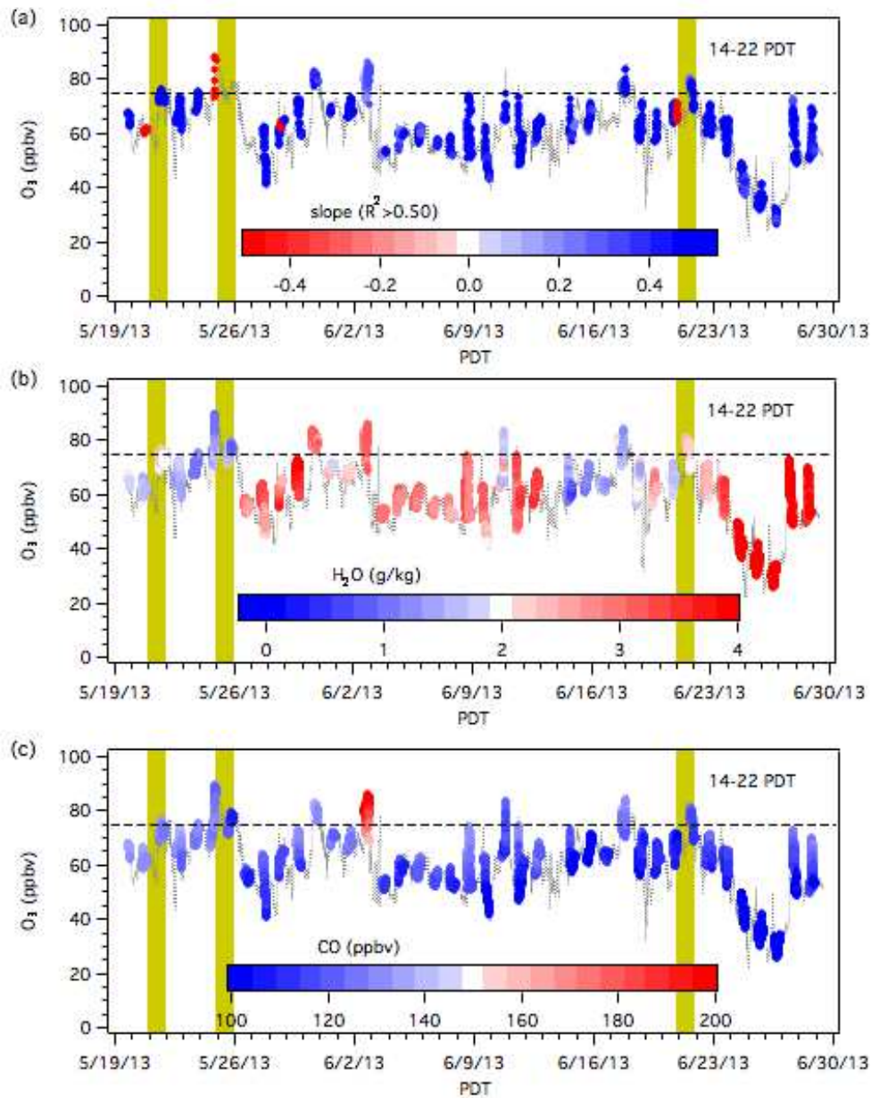
Figure 15. Time series of the in situ O_3 at Angel Peak color-coded by (a) the slope of the regression with CO ( R^2 > 0.5 only), (b) specific humidity, and (c) CO concentrations. The horizontal dashed line indicates the 75 ppbv 8-h NAAQS. The yellow bands mark the three exceedance days in Clark County.
