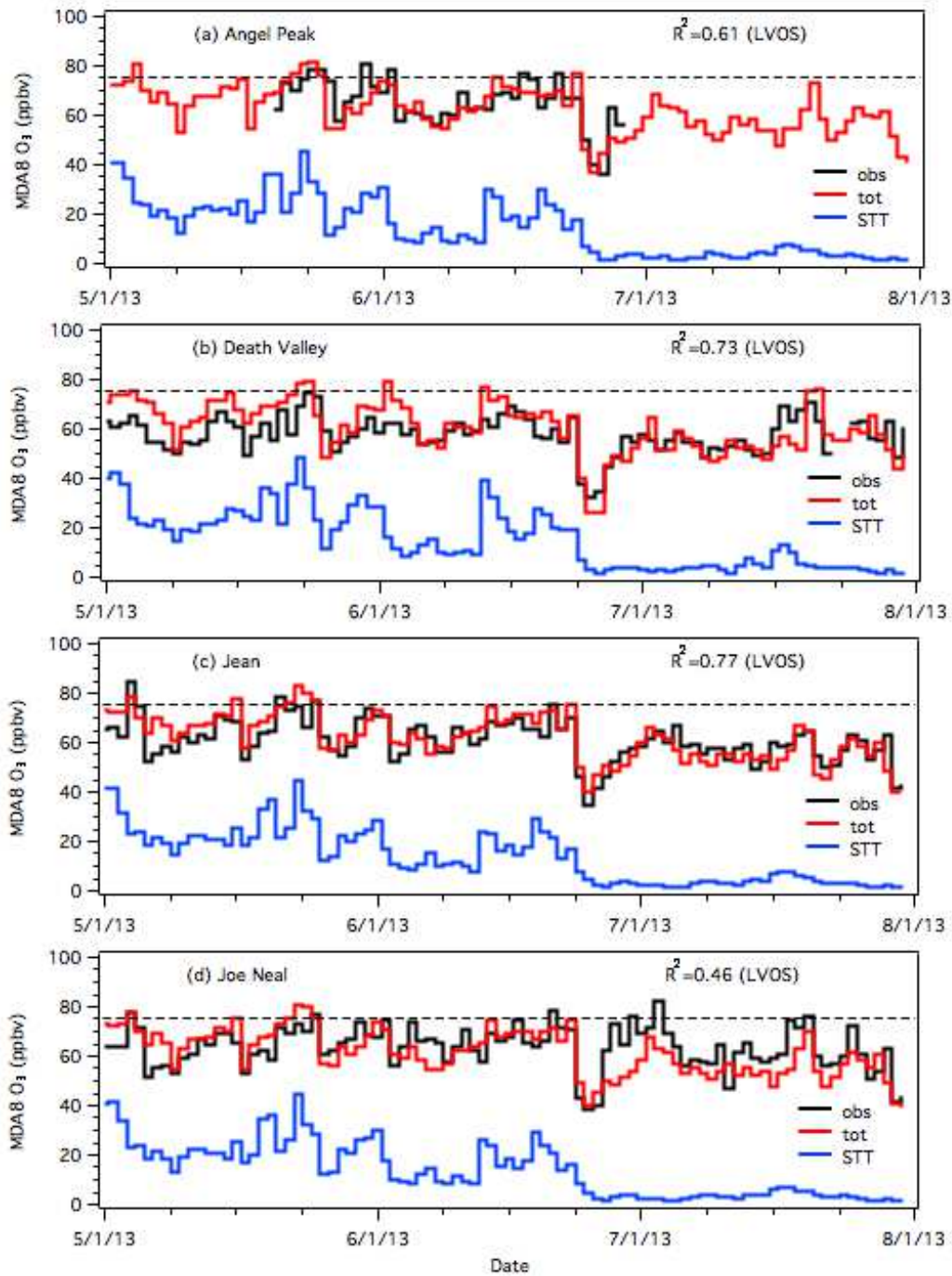
Figure 17. Time series comparing the AM3 total MDA8 ozone (red) calculated for (a) Angel Peak, (b) Death Valley, (c) Jean, and (d) Joe Neal to the measured values (black). The blue traces isolate the STT contribution to the calculated totals. The correlation coefficients are derived from linear regression fits using the data from May 19 to June 28 (LVOS) only.
