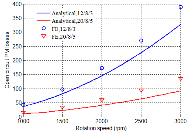
Fig. 6. Open circuit PM losses.
