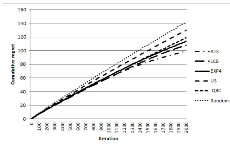
Fig. 2. Cumulative Regret for Active learning algorithms
