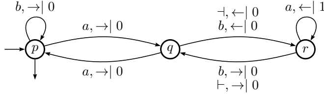
Figure 1: The two-way \mathcal{N} -automaton \mathcal{A}_1 .
