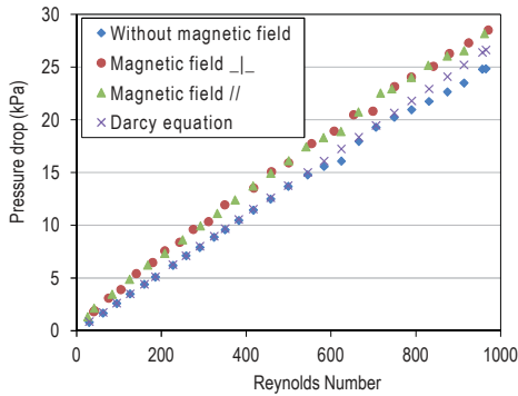
Figure 6: Pressure drops at different Reynolds numbers
