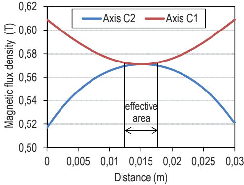
Figure 4: Y component of the magnetic flux density in the air gap
