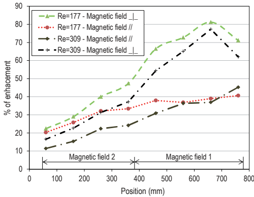
Figure 10: Influence of the magnetic field location: % of enhancement = [h(\text{with magnet}) - h(\text{without magnet})] / h(\text{without magnet})
