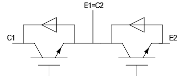
Figure 11: Electrical schematic of power module
