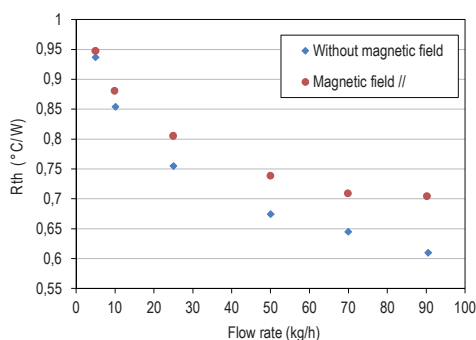
Figure 13: Thermal resistance of diode 1
