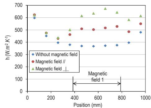
Figure 7: Local convective heat coefficient for Re=177 with magnetic field 1
