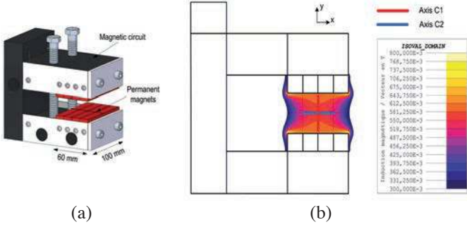
Figure 3: The magnetic sources (a) dimensions, (b) mapping of magnetic flux density in air gap of 34 mm.
