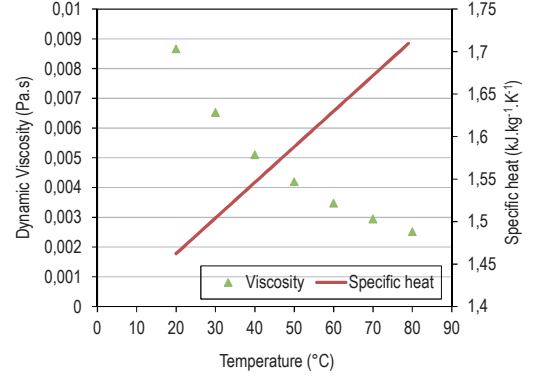
Figure 5: Specific heat and viscosity of EFH-1 without magnetic field
