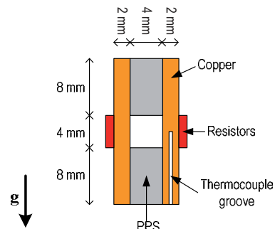
Figure 2: Cross section of the test section
