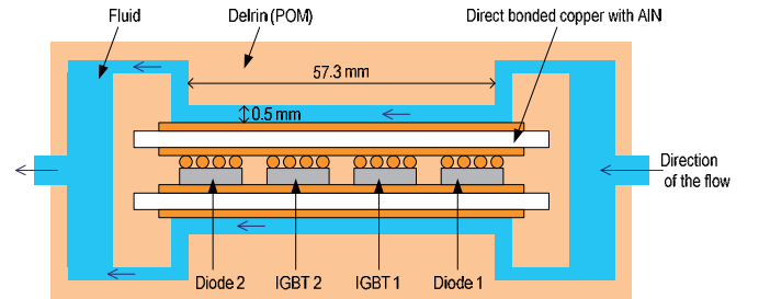
Figure 12: Schematic cross section of the power module
