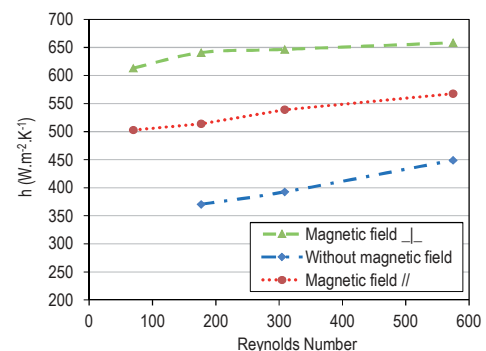
Figure 8: Variation of the average convective heat transfer coefficient with the Reynolds number (magnetic field 1)
