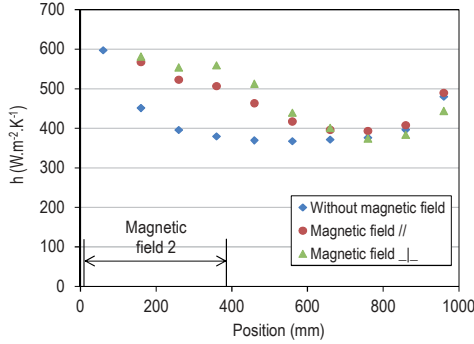
Figure 9: Local convective heat coefficient for Re=177 with magnetic field 2 located in thermally developing flow
