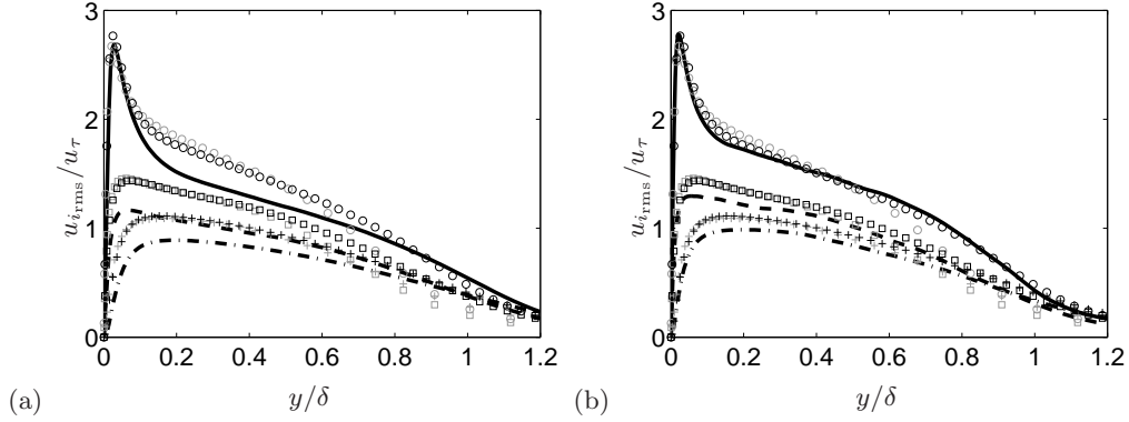
FIGURE 4. Turbulent intensities: u_{1,\text{rms}}/u_{\tau} (— present LES; \circ Spalart; \square Jimenez), u_{2,\text{rms}}/u_{\tau} ( \cdots present LES; + Spalart; + Jimenez), u_{3,\text{rms}}/u_{\tau} (--- present LES; \square Spalart; \square Jimenez). (a) coarse-grid LES results at x_1/\delta_{\text{ref}}=79.1 , and (b) fine-grid LES results at x_1/\delta_{\text{ref}}=73 .
