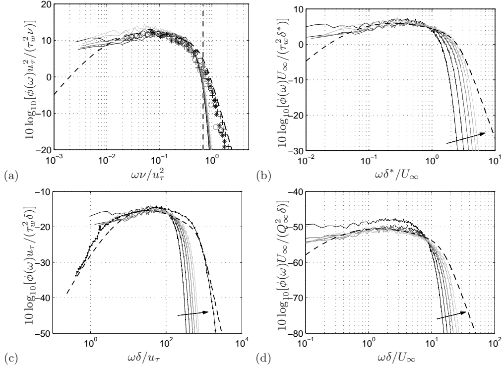
FIGURE 13. Frequency power spectra of wall pressure for successive streamwise abscissae: — x_1/\delta_{ref}^*=75.9 ( Re_\theta=848 ); — x_1/\delta_{ref}^*=151.8 ( Re_\theta=1180 ); — x_1/\delta_{ref}^*=227.8 ( Re_\theta=1491 ); — x_1/\delta_{ref}^*=303.7 ( Re_\theta=1781 ); — x_1/\delta_{ref}^*=379.6 ( Re_\theta=2058 ); — x_1/\delta_{ref}^*=455.6 ( Re_\theta=2328 ). (a) Scaling by inner variables: \tau_w as pressure scale and \nu/u_\tau^2 as timescale. Experimental spectra are superimposed: ++ Gravante et al. (1998) ( Re_\theta=2953 ); ** Farabee & Casarella (1991) ( Re_\theta=2945 ); oo Schewe (1983) ( d=2 mm, Re_\theta=1400 ); oo Schewe (1983) ( d=4 mm, Re_\theta=1400 ). The semi-empirical model of Goody (2004) for R_T=20 is plotted with a black dashed line, and the vertical dashed line indicates the frequency cut-off of the LES. (b) Scaling by outer variables: \tau_w as pressure scale and \delta_{ref}^*/U_\infty as timescale. The arrow show the increasing longitudinal locations. - - -: Goody's model ( R_T=20 ). (c) Scaling by outer variables: \tau_w as pressure scale and \delta_{ref}/u_\tau as timescale. The measurements of Farabee & Casarella (1991) for U_\infty=15 m/s are superimposed (•••), along with Goody's model for R_T=47.11 (— —). (d) Scaling by outer variables: the dynamic pressure Q_\infty = \frac{1}{2}\rho_\infty U_\infty^2 as pressure scale and \delta_{ref}/U_\infty as timescale. - - -: Goody's model ( R_T=20 ).
