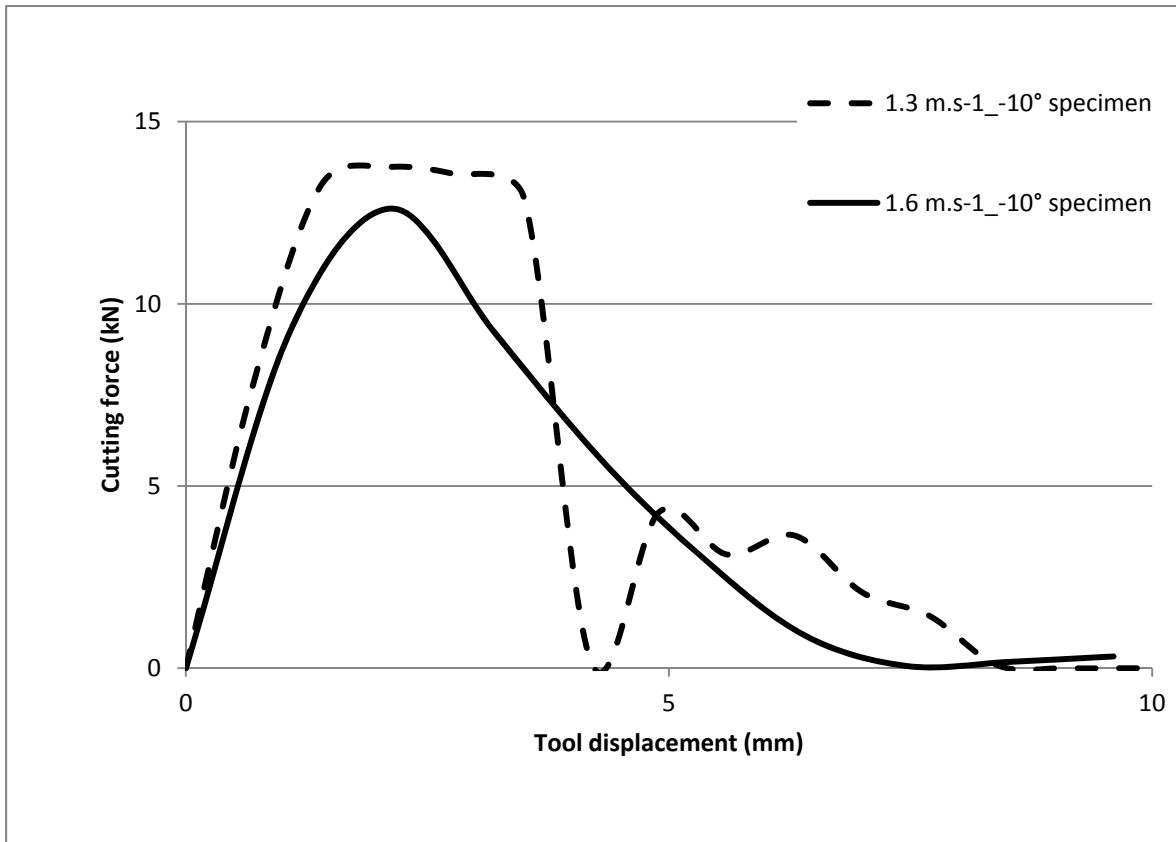
Figure 12. Experimental cutting force-displacement curves for both 1.3\text{ m}\cdot\text{s}^{-1}_{-10^\circ} and 1.6\text{m}\cdot\text{s}^{-1}_{-10^\circ} specimens. [ h=15\text{mm} and \phi=10\text{mm} ].
