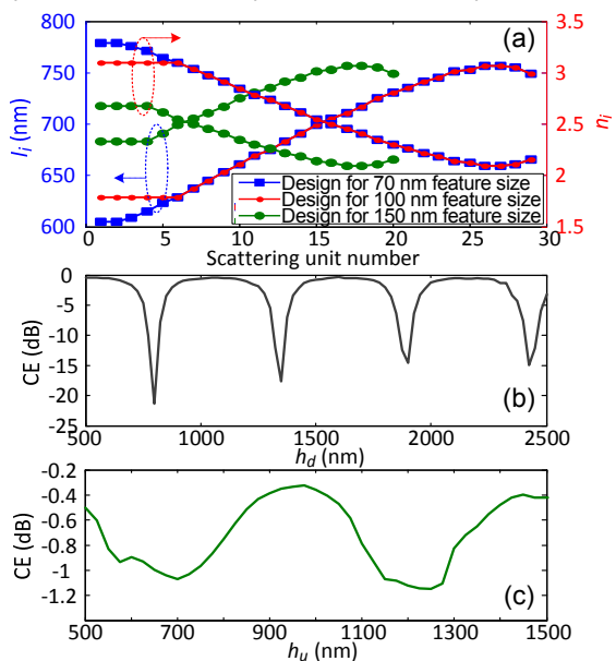
Fig. 2: (a) Designed l_i and n_i distributions of the grating couplers with feature sizes of 70 nm, 100 nm, and 150 nm. Simulated coupling efficiency as a function of (b) lower cladding thickness with h_u=1000 nm, and (c) upper cladding thickness with h_d=1600 nm.
