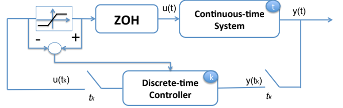
Fig. 1. Closed-loop system.
