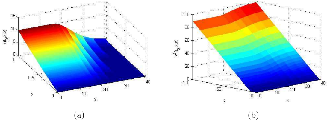
Figure 3: Surface of v(t, x, p) and v^\sharp(t, x, q) at t = t_0 .
