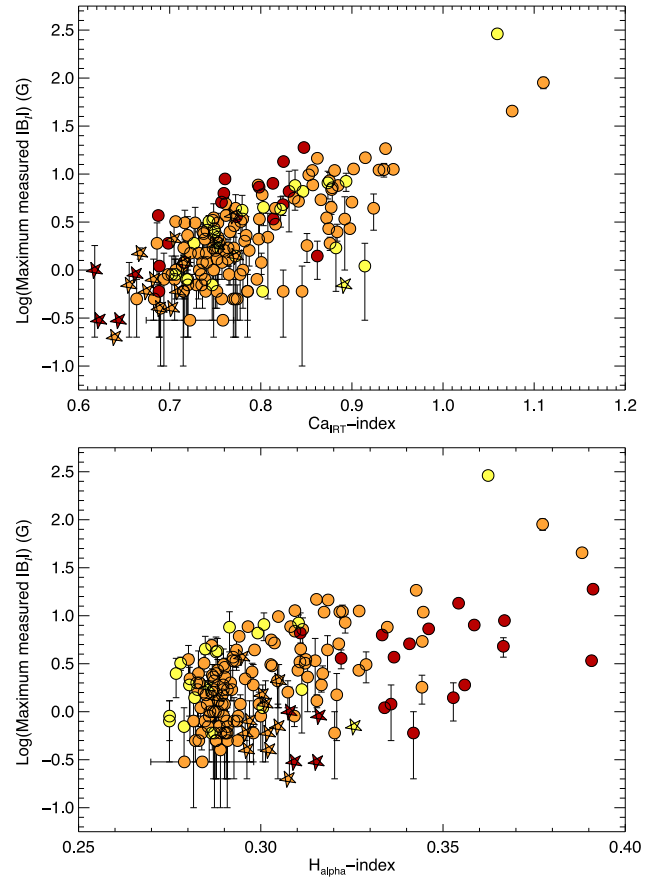
Figure 16. Plot of \log(\text{maximum measured } |B_l|) against the \text{Ca}_{IRT} activity index (top) and the H\alpha activity index (bottom). The symbols are the same as in Fig. 1.
