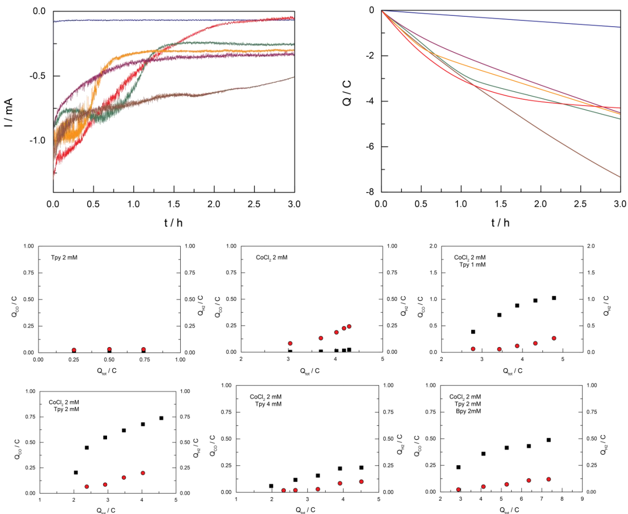
Figure S19. Top: current (left) and charge (right) measured during controlled-potential electrolyses of CO 2 -saturated solutions at -2.03 V of: 2 mM tpy (blue), 2 mM CoCl 2 (red), 2 mM tpy and 2 mM CoCl 2 (yellow), 4 mM tpy and 2 mM CoCl 2 (purple), 1 mM tpy and 2 mM CoCl 2 (green) and a mixture of 2 mM CoCl 2 , 2 mM tpy and 2mM bpy (brown). Data was recorded every 0.2 s and the current intensity data was smoothed using an adjacent-averaging method over 4 s. Bulk electrolyses were performed in 10 mL of DMF/H 2 O (95:5, v:v), with 0.1M TBAP, using a 1.5 cm diameter pool of mercury as the working electrode. The cell used is described in Figure S20. Bottom: charge corresponding to the products measured (CO: black squares, H 2 : red circle) vs. the total charge passed during the electrolyses.
