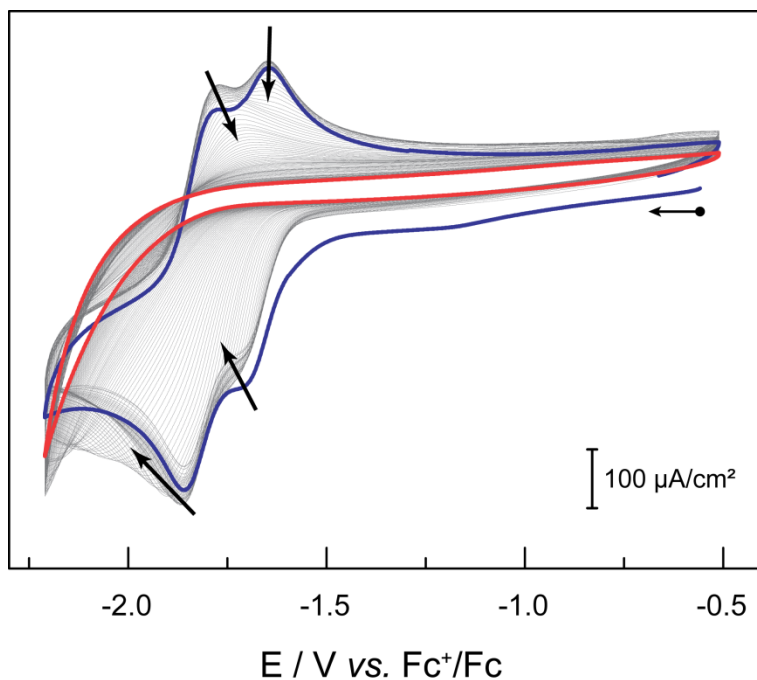
Figure S7. Cyclic voltammograms of a 2 mM N 2 -saturated solution of Zn-tpy and its evolution as the number of scans is increased. The working electrode used was 1 mm diameter glassy carbon electrode, the counter electrode was a platinum wire, and the reference electrode was a Ag/AgCl, 3M KCl reference electrode. The solvent system used was DMF/H 2 O (95:5, v:v), with 0.1M of TBAP as supporting electrolyte. The first scan is represented in blue and the last scan in red. Arrows indicate the evolution of the electrochemical features.
