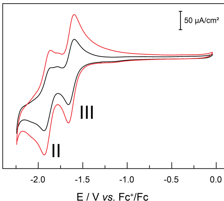
Figure S4. Cyclic voltammograms of a 2 mM N 2 -saturated solution of Ni-tpy at slow scan rates (10 mV/s, black; 20 mV/s, red). The working electrode used was 1 mm diameter glassy carbon electrode, the counter electrode was a platinum wire, and the reference electrode was a Ag/AgCl, 3M KCl reference electrode. The solvent system used was DMF/H 2 O (95:5, v:v), with 0.1M of TBAP as supporting electrolyte.
