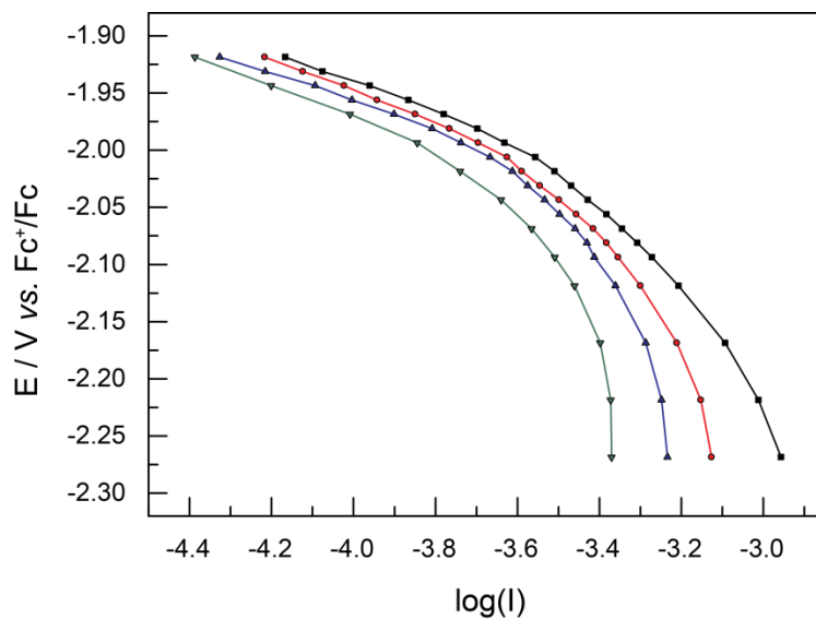
Figure S18. Plot of applied potential vs. \log(\text{current(A)}) extracted from the experiments described in Figure S17 (black squares: 2 mM, red circles: 1 mM, blue triangles: 0.75 mM and green triangles: 0.5 mM of Co-tpy ). At all Co-tpy concentrations, the slope of the linear fit (not represented) of the -1.9 V to -2.1 V region is \sim 135 mV/dec).
