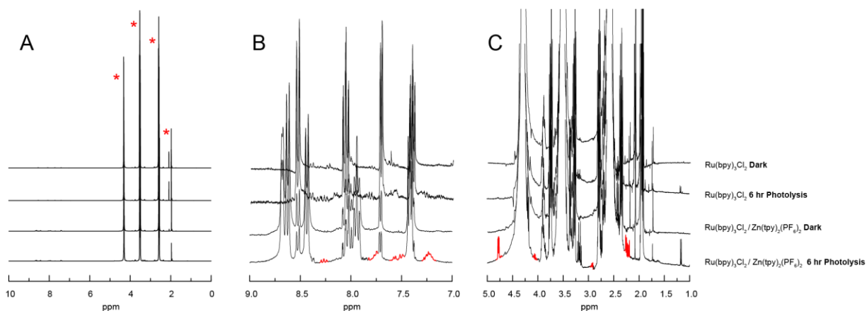
Figure S15. 1 H NMR spectra for the photolysis of experiments of 1.0 mM Zn-tpy in the presence of 2.0 mM Ru(bpy) 3 Cl 2 (H 2 O) 6 in a CO 2 -saturated 5:1 volumetric ratio of acetonitrile-d 3 to triethanolamine. (a-c) From top to bottom, the spectra represent Ru(bpy) 3 Cl 2 (H 2 O) 6 in the dark; Ru(bpy) 3 Cl 2 (H 2 O) 6 photolyzed; both Ru(bpy) 3 Cl 2 (H 2 O) 6 and Zn-tpy in the dark; and both Ru(bpy) 3 Cl 2 (H 2 O) 6 and Zn-tpy photolyzed. (a) The full spectra are shown with the intense peaks associated with TEOA marked by *. (b) Aromatic resonances are shown with peaks only observed post-photolysis of Zn-tpy presented in red. (c) Aliphatic resonances are shown with peaks only observed post-photolysis of Zn-tpy presented in red.
