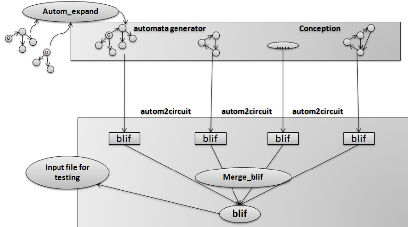
Fig. 9. Model Tool chain
