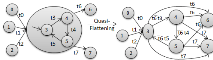
Fig. 3. Initial and Normal Transition Linking
