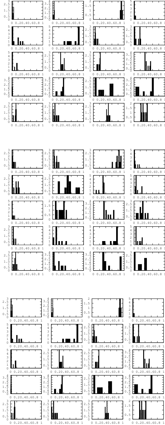
FIGURE 2. The optimization algorithm iterates from the initial guess (\mathcal{P}_0, \mu_0) and constructs a sequence of estimations (\mathcal{P}_k, \mu_k) . We plot here several histograms of the laws \mathcal{L}_Y(|(\Psi_1^{\epsilon_i}(T, Y))_j|^2) for various choices of k and i = 1, \dots, 5 and j = 1, 2, 3, 4 . In the top picture are the histograms of the observations for the real law, in the middle picture are the histograms for the initial guess k = 0 and in the bottom image the histograms for the final iteration k = 277 . The optimization worked well as there is an obvious match between the top and the bottom histograms.
