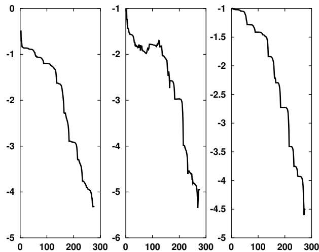
FIGURE 1. The logarithm of \mathcal{J} (left), the relative error on \mathcal{P} (middle) and the relative error on \mu (right) as a function of the iteration index.
