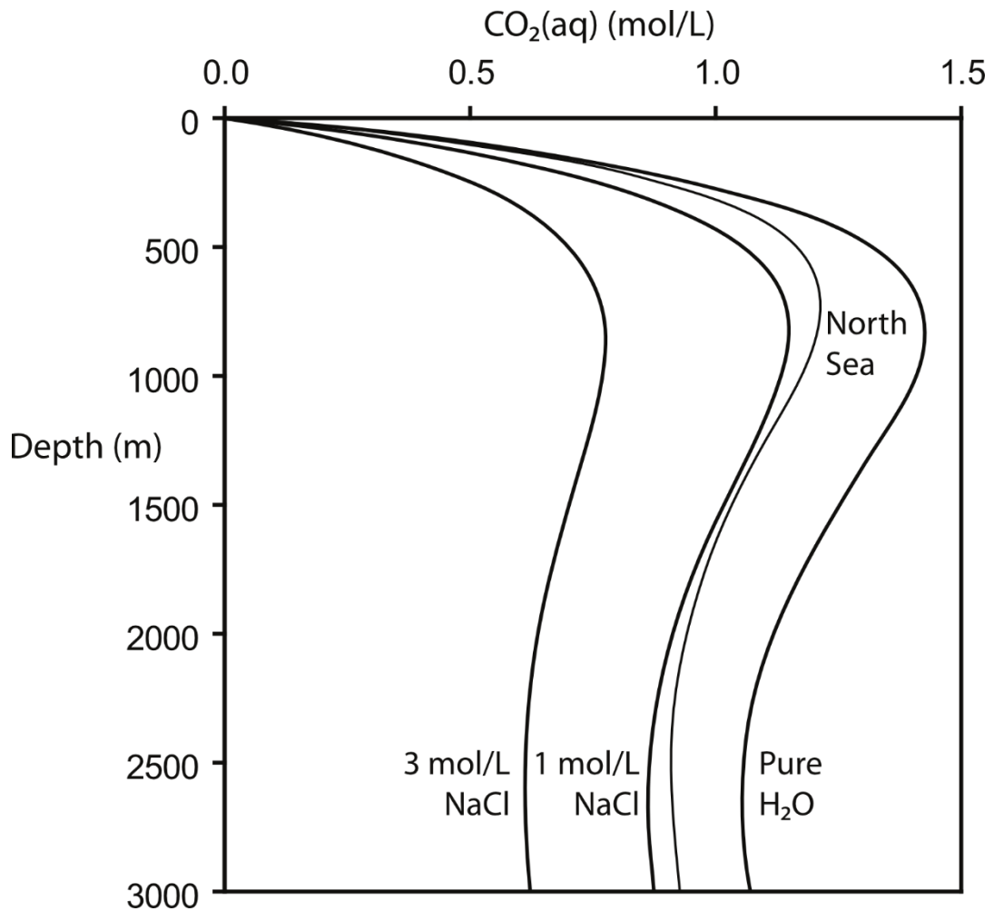
Figure 7 \text{CO}_2 solubility as a function of depth below surface. Solubility profiles calculated using equations from (Duan et al., 2006), considering typical geothermal gradients of 25^\circ\text{C}/\text{km} and hydrostatic pressure gradients, in pure water and fluid salinities of 1 mol/L and 3 mol/L NaCl. An example for a typical North Sea geothermal gradient of 25^\circ\text{C}/\text{km} and pore salinity profile of 25,000ppm/km (Bjørlykke and Gran, 1994) is also shown.
