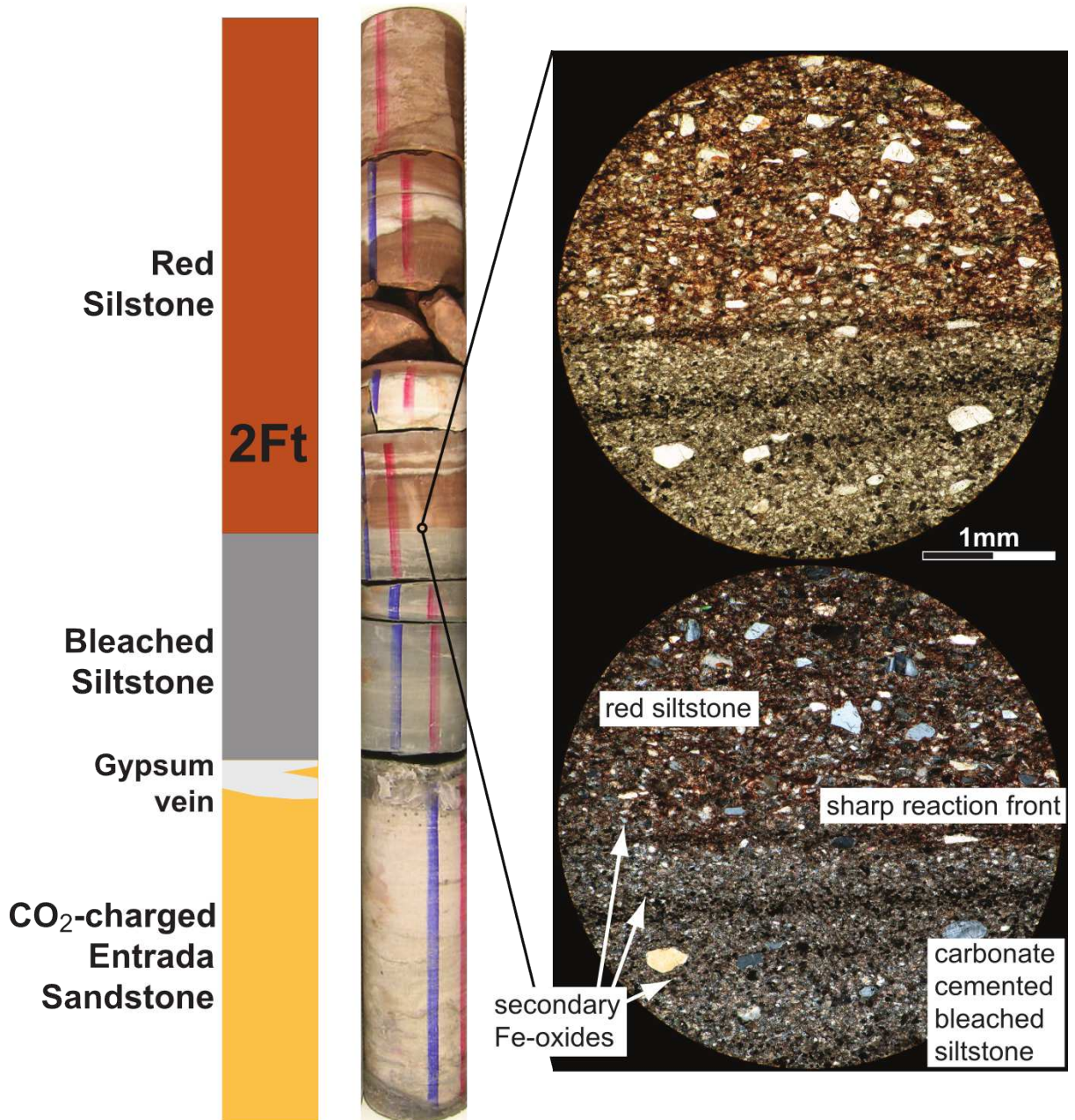
Figure 20 Core photograph from well CO2W55 showing the contact between CO 2 -bearing sandstone of the Entrada Sandstone and siltstone horizons that form internal seals to the CO 2 -charged fluids. The lower 10cm's of siltstone has been bleached by removal of Fe-oxide grain coatings by interaction with the CO 2 and micrographs from the bleached-unbleached contact show the mobilized Fe has been redeposited at the reaction front in bands of coarse Fe-oxides, along with abundant carbonate cement throughout the bleached interval. The short distance over which the siltstone has been bleached suggests that the CO 2 has penetrated the siltstone by diffusion and that reactions with the host rock have attenuated the reactivity of the CO 2 over this cm length scale. These observations suggest that fluid-mineral reactions help retard the diffusion distance of the CO 2 , potentially aided by the formation of carbonate cement that blocks pores, and that such siltstone layers can form impermeable barriers to the CO 2 and effective seals over 100,000 year time scales.
