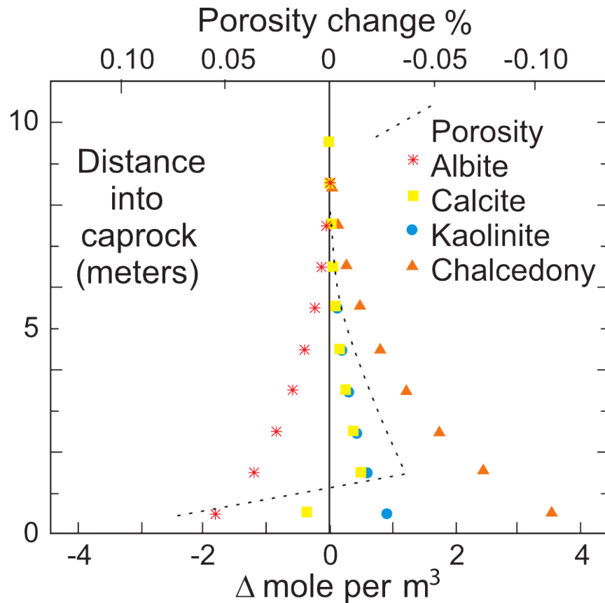
Figure 9 Alteration at the base of caprock by supercritical CO 2 , calculated from reactive transport modelling (redrawn after Gaus et al., 2005). Changes in mineral modes reflect dissolution of albite and precipitation of kaolinite and chalcedony throughout the profile, and dissolution of calcite at the base of the profile but precipitation greater than ~ 1 m above the base. Note the net decrease in porosity except at the very base of the profile. Redrawn after Gaus et al., (2005).
