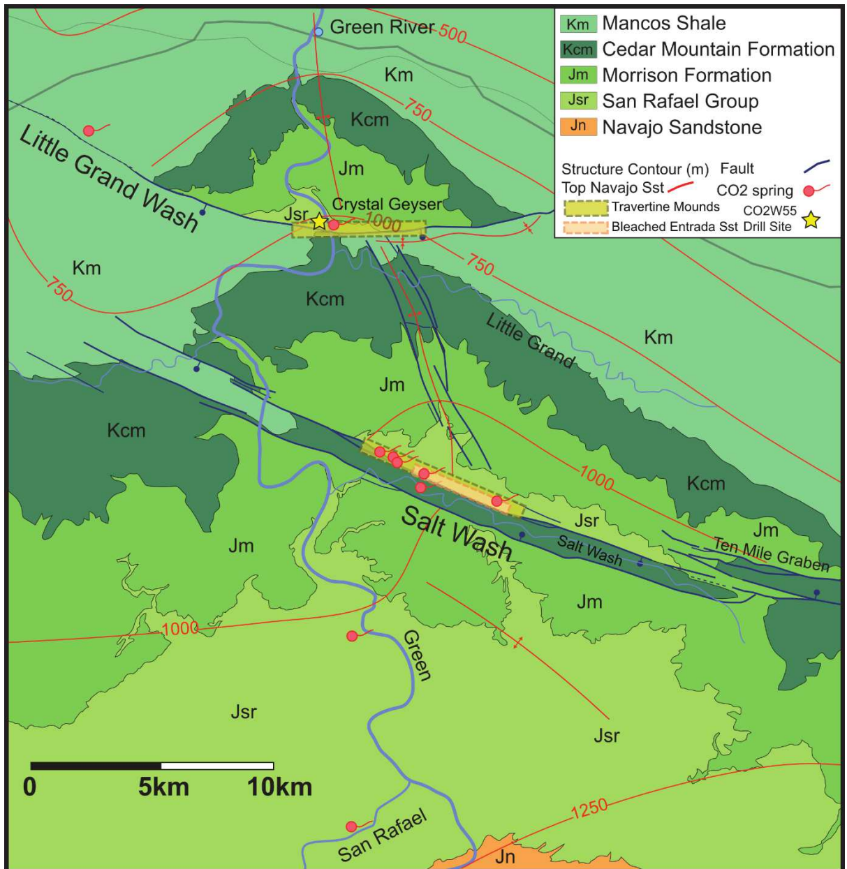
Figure 18 Geological map of the Green River anticline showing locations of the Little Grand Wash and Salt Wash Graben normal fault systems, CO 2 -springs and location of drill hole CO2W55 (redrawn after Kampman et al., 2009). Supercritical CO 2 is buoyantly accumulated within the White Rim sandstone (>800m depth) at the anticline crest in traps formed by the faults, which are laterally sealing due to shale and clay gauge cores (Dockrill et al., 2010). The faults contain a damage zone of open fractures that allows CO 2 and CO 2 -charged brine to migrate vertically, filling a series of shallow sandstone reservoirs in the Wingate, Navajo and Entrada Sandstones. The CO 2 and CO 2 -charged brines mix with
