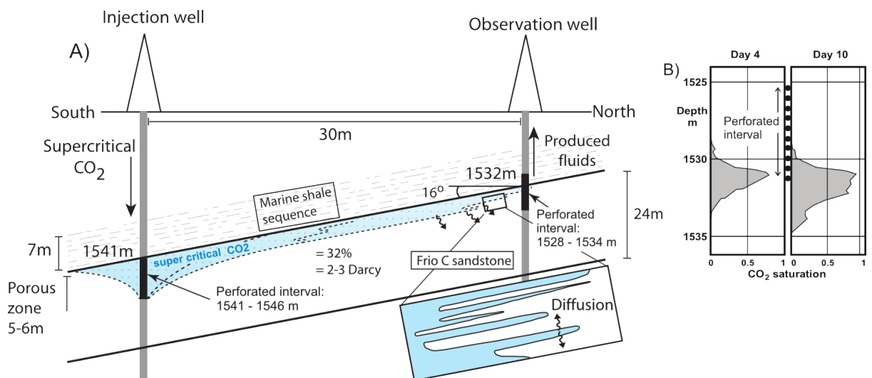
Figure 10 The Frio-I injection experiments involved injection of 1600 tonnes of supercritical CO 2 at a depth of 1500m into the Upper Frio Formation, over 11 days. The injection experiment utilised a U-tube sampling line in a single observation well sited 30m to the north and at ~ 9m higher elevation with a 6 m perforated interval. This was used to monitor changes in in-situ fluid density and gas phase compositions and to recover single and two-phase fluid samples for chemistry and stable isotope measurements. Fluid pH was
