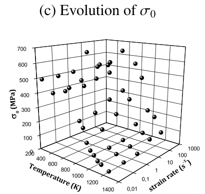
Fig. 10. Example of the evolution of the parameters \sigma_s , \sigma_0 , r , A , and n as a function of T and \dot{\varepsilon} – for the 42CrMo4-BA steel.
