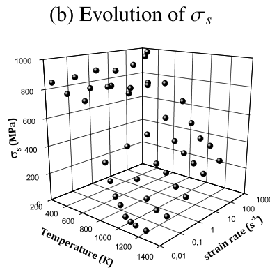
Fig. 10. Example of the evolution of the parameters \sigma_s , \sigma_0 , r , A , and n as a function of T and \dot{\varepsilon} – for the 42CrMo4-BA steel.
