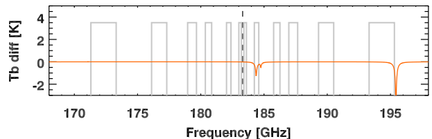
FIG. 5. The BT difference between simulations with MonoRTM, including ozone minus simulations without ozone (orange line) for a tropical standard atmosphere and zenith angle of 42^\circ . The gray boxes show the SAPHIR channels' positions and widths.
