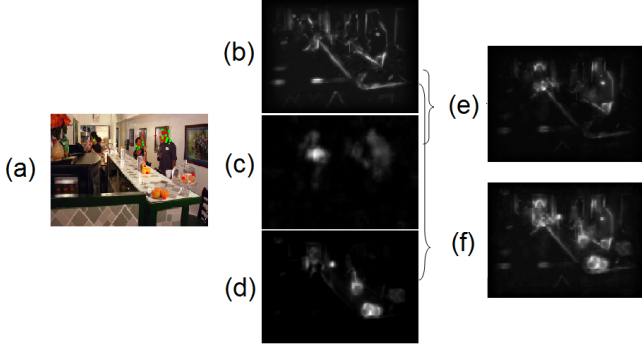
Fig. 2: An example frame and its corresponding saliency maps, (a) Original frame (b) luminance saliency map M_{ls} , (c) dynamic saliency map M_{id} , (d) chrominance M_{cs} , (e) fusion of M_{ls} and M_{id} , (f) fusion of M_{ls} , M_{cs} and M_{id} .
