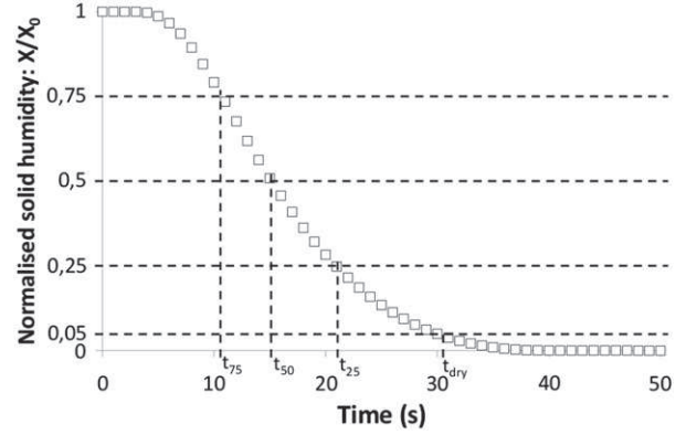
Fig. 7. Definition of the characteristic times.
