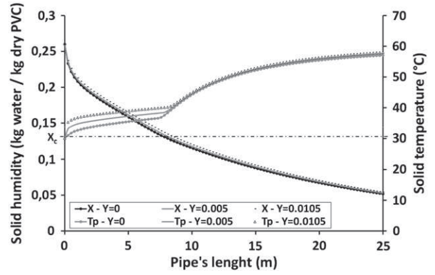
Fig. 25. Evolution of solid humidity and temperature versus pipe length for different inlet air humidity.
