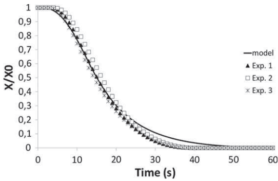
(b) Evolution of PVC normalised humidity versus time
