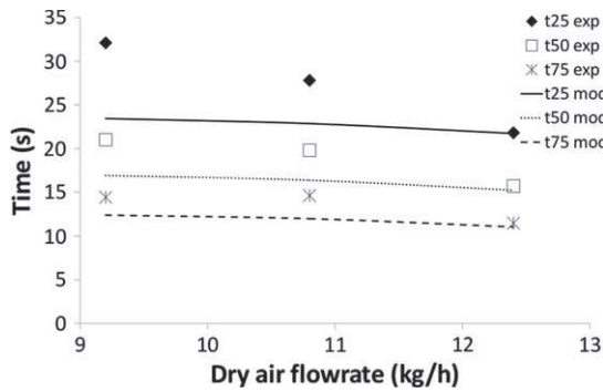
(c) Influence of the dry air flowrate
