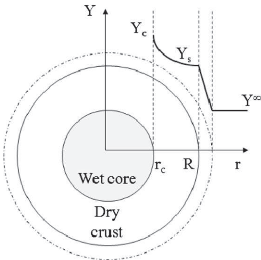
Fig. 13. Shrinking core model.
