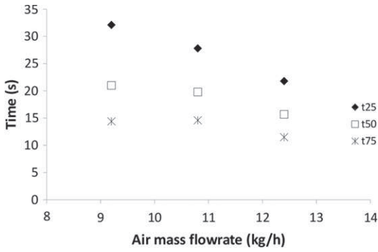
(b) Evolution of characteristic times versus air mass flowrate
