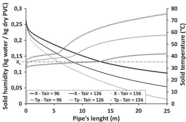
Fig. 24. Evolution of solid humidity and temperature versus pipe length for different inlet temperatures: 126, 96, and 156 °C.
