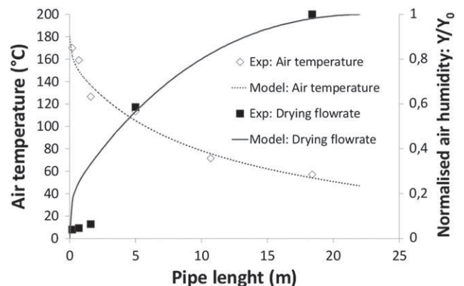
Fig. 22. Comparison between numerical results and INEOS industrial data.
