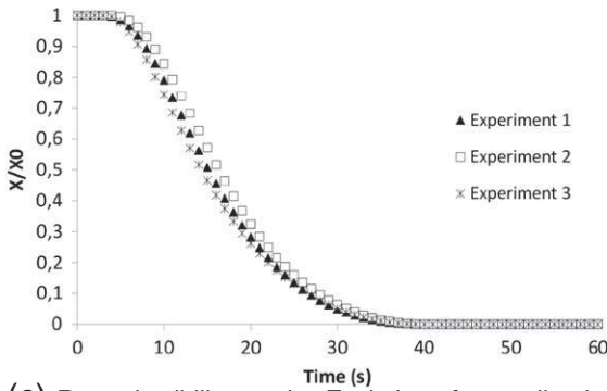
(c) Reproducibility results: Evolution of normalised solid humidity (Exp. 1, 2, & 3)
