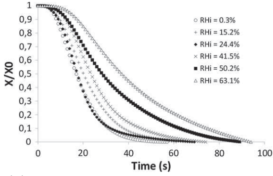
(a) Evolution of the normalized solid humidity versus time
