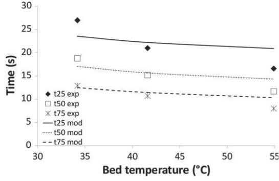
(a) Influence of the bed temperature
