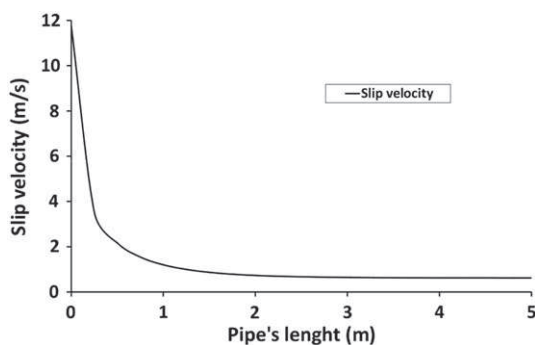
Fig. 20. Evolution of slip velocity versus pipe length.
