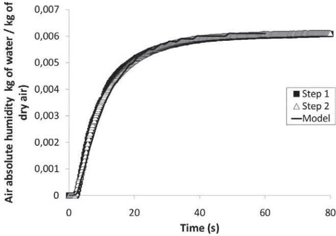
(a) Comparison between numerical and experimental results
