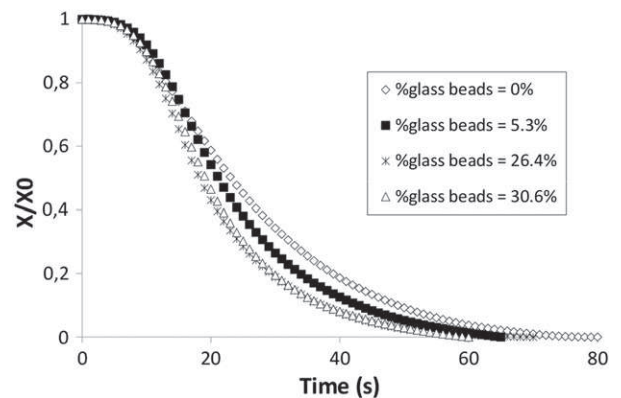
Fig. 8. Evolution of solid humidity for different fraction of glass beads. Air velocity: 32.3 cm/s; T_{bed} = 34.2 °C; cake weight: 2.9 g.
