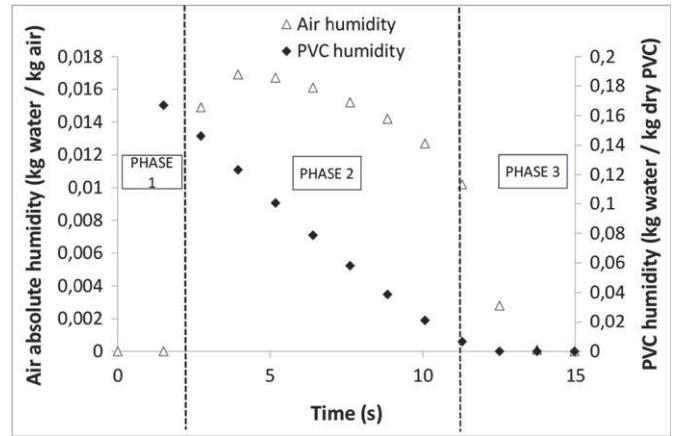
(a) Evolution of air absolute humidity and PVC humidity
