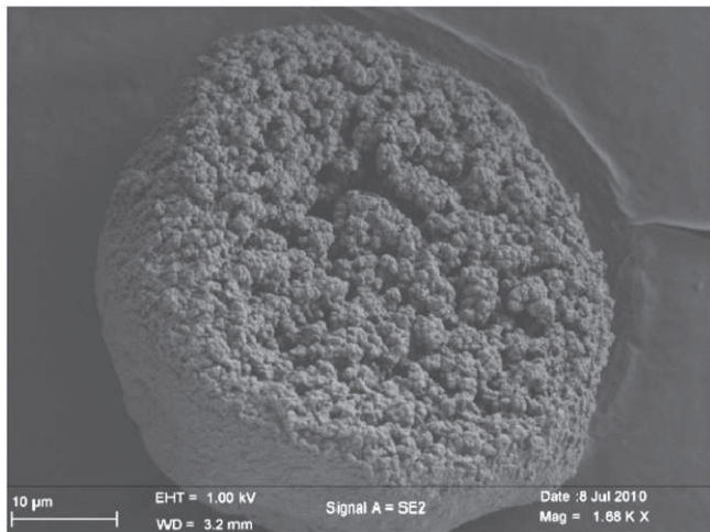
Fig. 4. SEM picture of a PVC particle.
