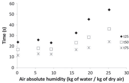
(b) Evolution of characteristic times versus inlet air absolute humidity
