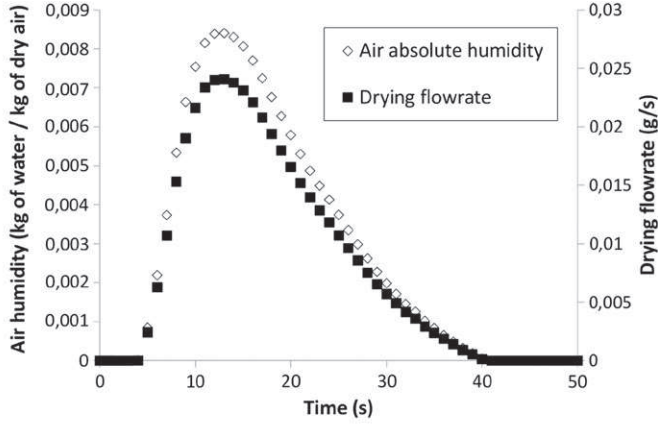
(a) Absolute air humidity & drying flowrate evolution (Exp. 1)
