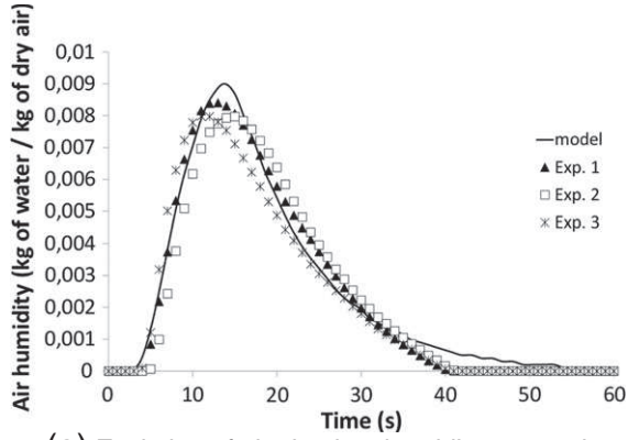
(a) Evolution of air absolute humidity versus time
