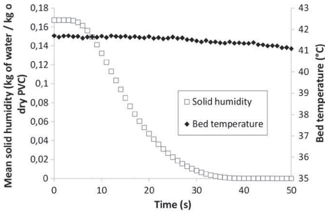
(b) Solid humidity and bed temperature evolution (Exp. 1)
