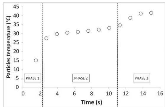
(b) Evolution of particle temperature
