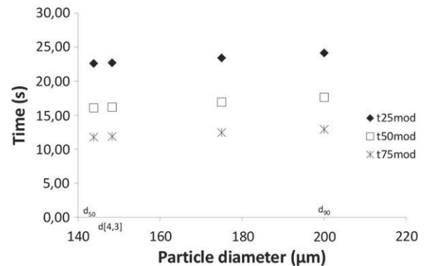
Fig. 17. Influence of particle diameter on the characteristic times.
