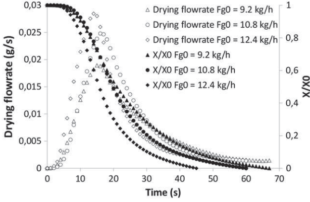
(a) Evolution of drying flowrate and normalised solid humidity versus time
