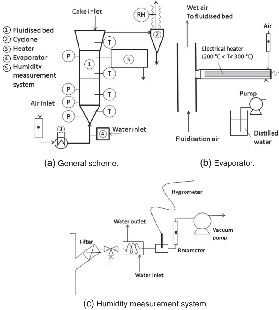
Fig. 5. Experimental pilot.
