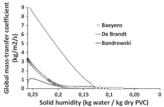
Fig. 21. Evolution of global mass transfer coefficient versus solid humidity for different correlations.
