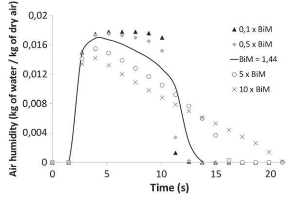
Fig. 16. Air absolute humidity evolution versus time for different Biot number values.
