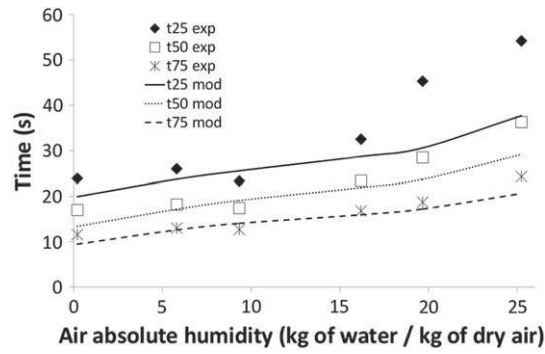
(b) Influence of the air inlet humidity
