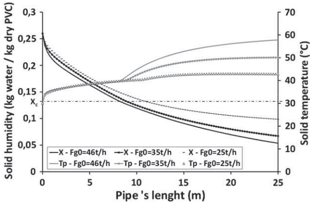
Fig. 23. Evolution of solid humidity and temperature versus pipe length for different dry air flowrates: 46.4, 35, and 25 t/h.
