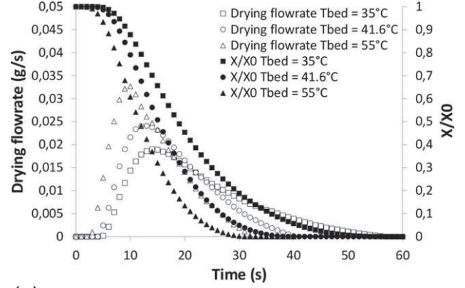
(a) Evolution of drying flowrate and normalised solid humidity versus time
