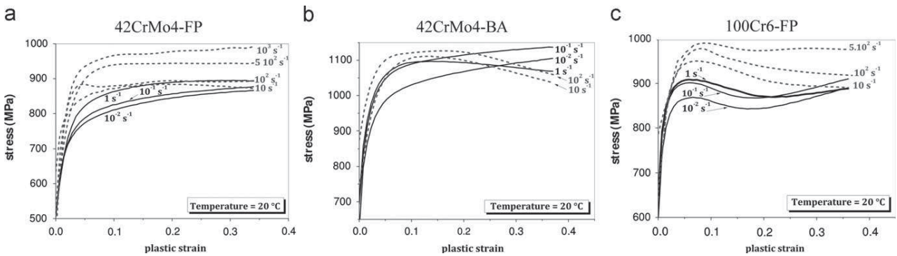
Fig. 10. Evolution of the compressive stress as a function of the plastic strain at 20\text{ }^{\circ}\text{C} for different strain rates. Comparison between the three steels studied.
