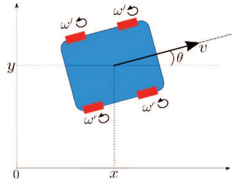
Fig. 3. Robot motion model.
