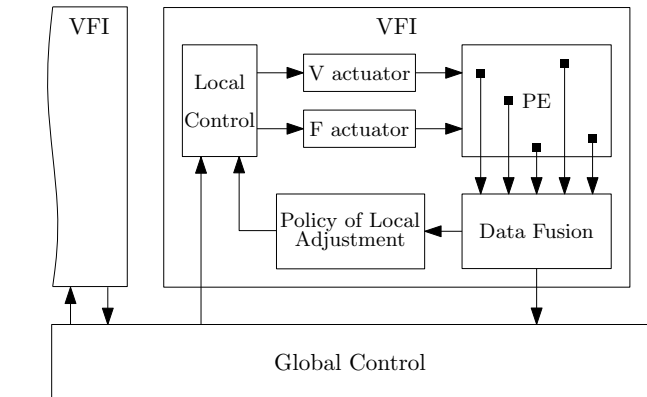
Fig. 1: Principle of an Adaptive Voltage and Frequency Scaling architecture. Each black square represents a sensor.
