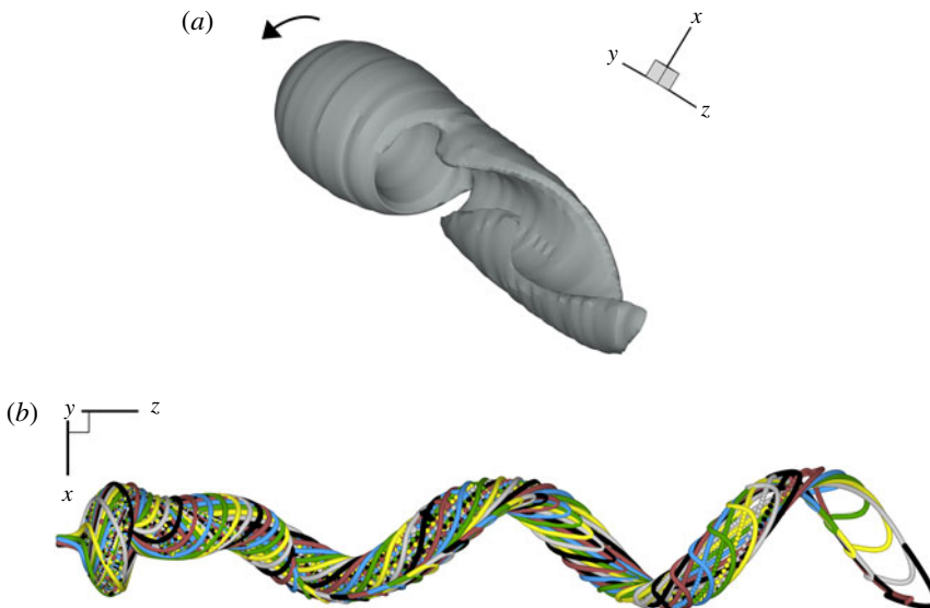
FIGURE 12. (Colour online available at journals.cambridge.org/flm ) Visualization of the stable simple helix at Re = 120 , S = 1.3 , based on the second-order analytic solution reconstructed from (5.1). (a) Isosurface of azimuthal vorticity \xi = -1.15 . The black arrow indicates the swirling direction of the ambient flow. (b) Numerically computed dye lines at t = 70 (see supplementary movie 1 for an animation). In (b), the scale is doubled in the axial direction.
