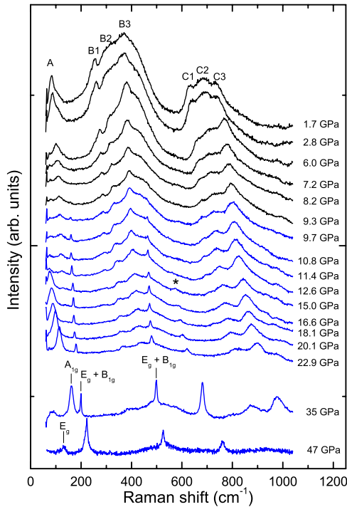
FIG. 5. (Color online) Selection of Raman spectra recorded as a function of pressure at room temperature.
