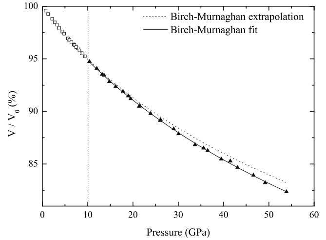
FIG. 3. Evolution of the relative volume with pressure at room temperature. The volume at ambient pressure [ V_0=59.66(1) \text{ \AA}^3 ] is taken from the fit to the Birch-Murnaghan EoS. The extrapolation calculated using the Birch-Murnaghan EoS is shown (dotted line), as well as the Birch-Murnaghan fit to the data in the tetragonal phase (solid line).
