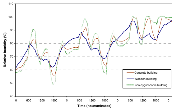
Figure 11 : Change of relative humidity inside the room for the three buildings.
