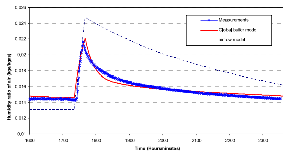
Figure 5 : Validation of global buffer model in the LGI test cell
