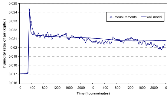
Figure 6 : Validation of wall model in the “STATron” test cell
