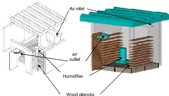
Figure 3 : LGI test cell for buffer model validation
