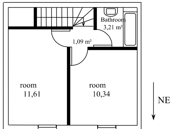
Figure 8 : Building under study.
