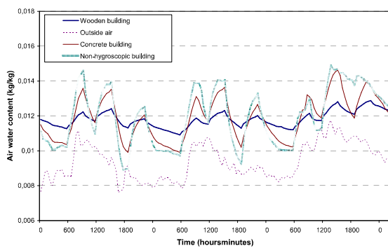
Figure 10: Change of air water content inside the room for the three buildings.
