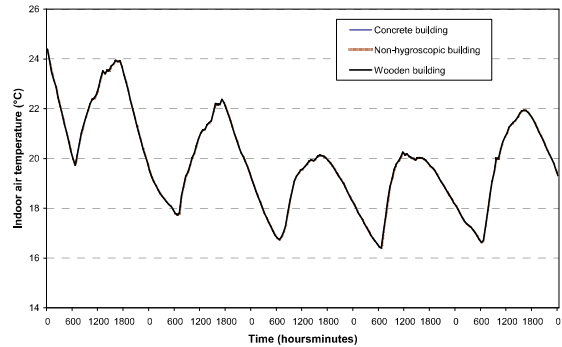
Figure 12: Evolution of indoor air temperature for the three buildings.
