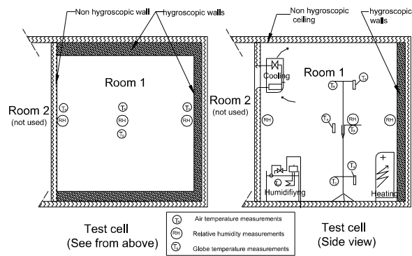
Figure 4 : Test cell called “STAttron” (side view and above)
