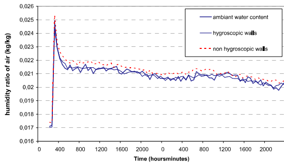
Figure 7 : Evolutions of water content of air in the room and nearby hygroscopic and non-hygroscopic walls
