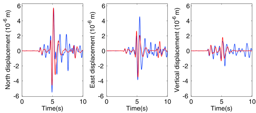
Figure 12. Comparison between displacements recorded at the ISPT station (blue) and synthetics (red), for the 27 August 2010, 08 h, 57 min, 15 s, event (see raw data in Figure 9). Both data and synthetics are band-pass filtered between 1 Hz and 2.5 Hz. This earthquake has been located at (latitude, longitude, depth) = (1.19°S, 81.02°W, 9.5 km) by the location procedure. The source parameters corresponding to synthetics are (strike, dip, rake) = (13°, 9°, 80°) and M_w = 3 . The good agreement between data and synthetics shows that this earthquake is consistent with a thrust mechanism along the subduction interface.
