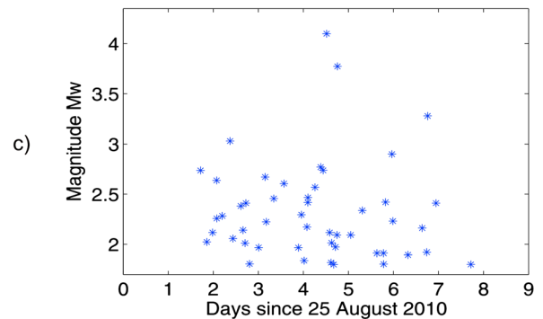
Figure 11. Magnitude and time distribution of the associated seismicity. (a) Map location, with color scaled to occurrence date and size to moment magnitude ( M w ). The smallest circles are events of M w =1.8, and the largest one is a M w =4.1 earthquake. The depth of the subduction interface is contoured and labeled (in km) as in Figure 3. (b) Gutenberg-Richter law with the classical b-value slope (equal to 1) presented on the left part of the figure. (c) Distribution of magnitude as a function of occurrence time.
