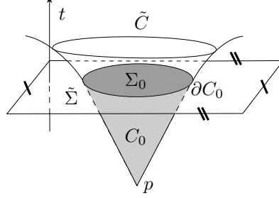
Fig. 1: The modified cone \tilde{C} .
