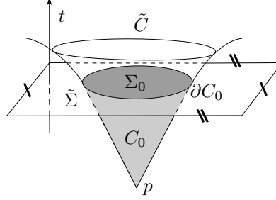
Fig. 1: The modified cone \tilde{C} .
