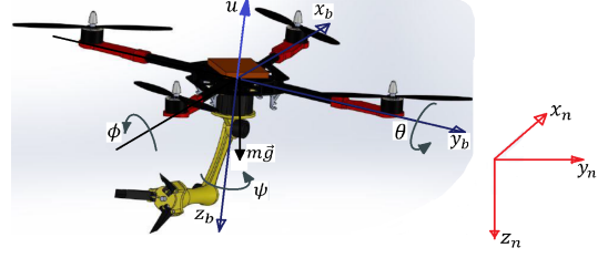
Fig. 2. Schematic configuration of a quadrotor carrying a manipulator arm.
