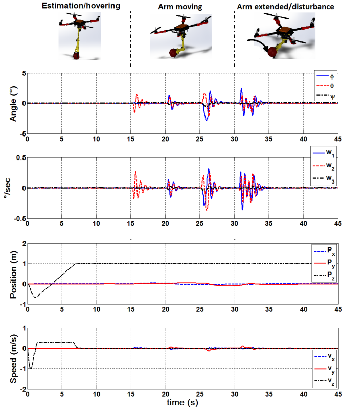
Fig. 3. Angular and linear position and velocity during the simulation.
