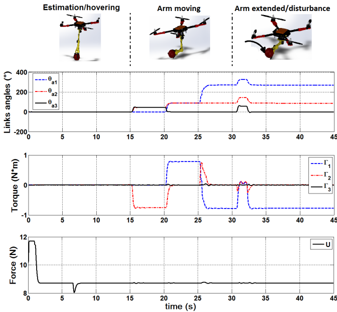
Fig. 4. Angular positions of the links of the manipulator, control torques and thrust signals during the simulation.
